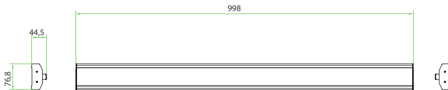
measure rail
